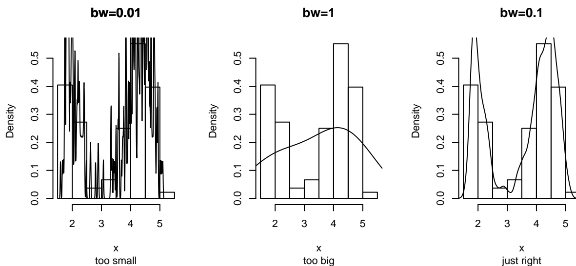
Figure 9: Histogram and density estimates. Notice choice of bandwidth is very important.
