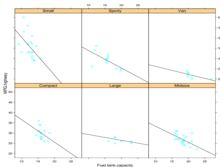
Figure 24: Example of lattice graphics: relation of m.p.g. and fuel tank size.
