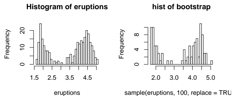
Figure 29: Bootstrap sample
