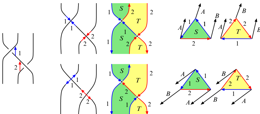
Figure 6: The tetrahedral decomposition of S^3 - (W(3, 1) \cup B)
