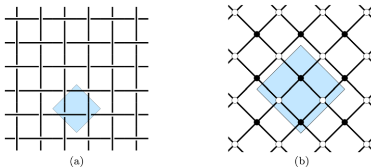
FIGURE 3 (colour online). (a) Infinite square weave \mathcal{W} and fundamental domain for \mathcal{W} . (b) Overlaid graph G_{\mathcal{W}}^b and fundamental domain for G_{\mathcal{W}}^b .
