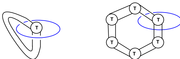
FIGURE 6 (colour online). Augmented hyperbolic alternating links K \cup B and K^m \cup B .
