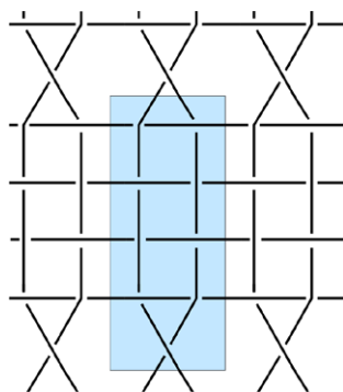
FIGURE 10 (colour online). Diagram for one of the biperiodic alternating links C_n , and fundamental domain for C_n . The link C_n as shown is for n = 3 .
