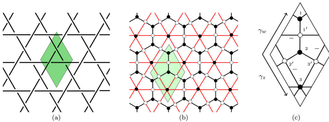
FIGURE 4 (colour online). (a) Diagram of biperiodic triaxial link \mathcal{L} , and fundamental domain for L . (b) Overlaid graph G_L^b and fundamental domain for G_L^b . (c) Toroidal graph G_L^b , with a choice of homology basis, ordered vertices and a choice of Kasteleyn signs on edges.
