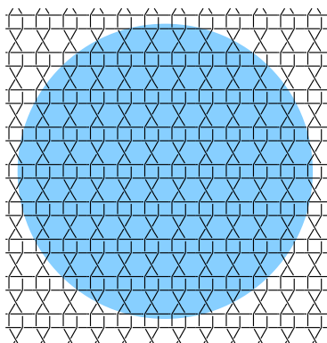
FIGURE 5 (colour online). Volume bound for Følner convergence of finite links K_n to a biperiodic link \mathcal{L} : the part G_n \subset G(\mathcal{L}) is shown in the disc. As G_n \subset G(K_n) , the bipyramid volume density of K_n converges to that of \mathcal{L} .
