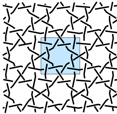
FIGURE 1 (colour online). A typical biperiodic alternating link.
