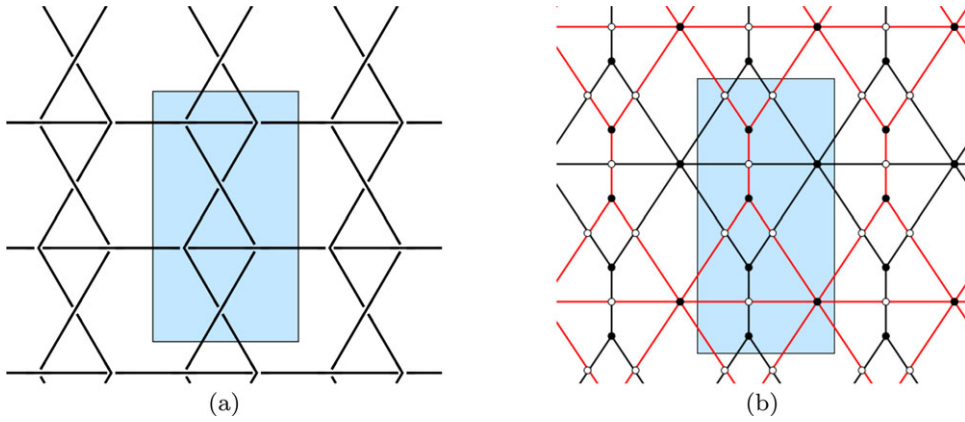
FIGURE 8 (colour online). (a) Diagram of biperiodic link C_0 , and fundamental domain for C_0 . (b) Overlaid graph G_{C_0}^b and fundamental domain for G_{C_0}^b .
