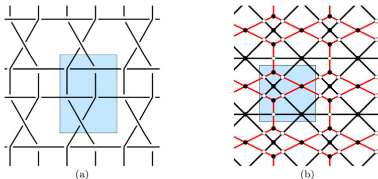
FIGURE 9 (colour online). (a) Diagram of biperiodic link C_1 , and fundamental domain for C_1 . (b) Overlaid graph G_{C_1}^b and fundamental domain for G_{C_1}^b .
