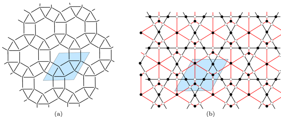
FIGURE 7 (colour online). (a) Diagram of the biperiodic Rhombitrihexagonal link \mathcal{R} , and fundamental domain for \mathcal{R} . (b) Overlaid graph G_{\mathcal{R}}^b and fundamental domain for G_{\mathcal{R}}^b .
