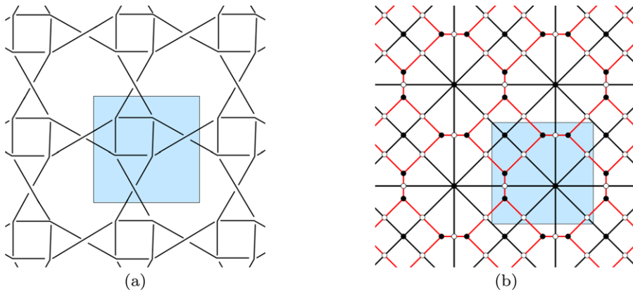
FIGURE 11 (colour online). (a) Diagram of biperiodic link \mathcal{K} , and fundamental domain for K . (b) Overlaid graph G_{\mathcal{K}}^b and fundamental domain for G_{\mathcal{K}}^b .
