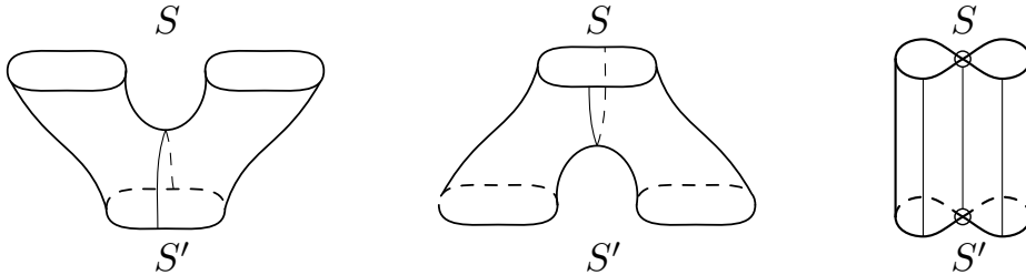
FIGURE 9. The three types of cobordisms from S to S' include a fusion (left), fission (middle), and single cycle smoothing (right).
