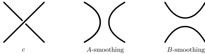
FIGURE 7. The A - and B -smoothing of a crossing.
