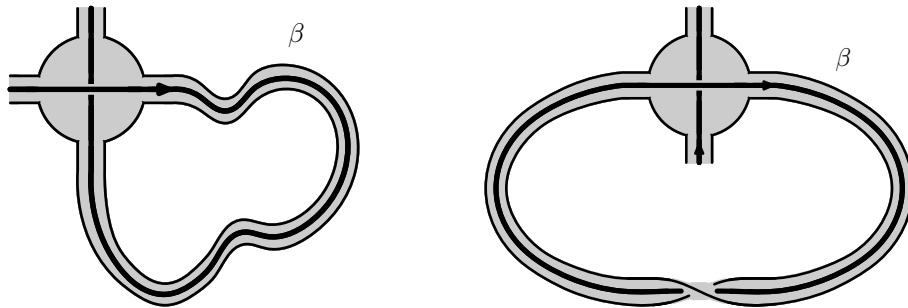
FIGURE 11. A flat band and a half-twisted band.
