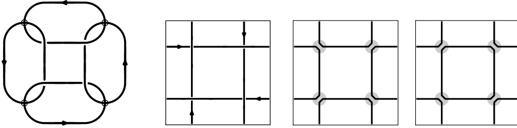
FIGURE 15. From left to right, a virtual link with four components, a minimal genus representative in the torus, and the states S_A and S_B .
