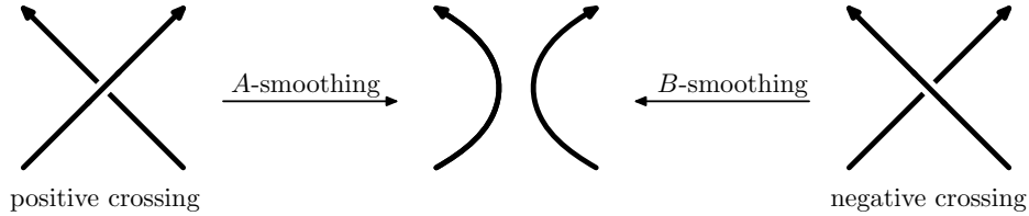
FIGURE 12. Oriented smoothings at positive and negative crossings.
