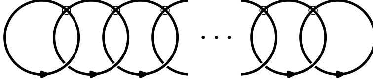
FIGURE 16. The virtual chain link.
