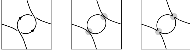
FIGURE 8. A minimal genus diagram of the virtual trefoil in the torus, and the states S_A and S_B .
