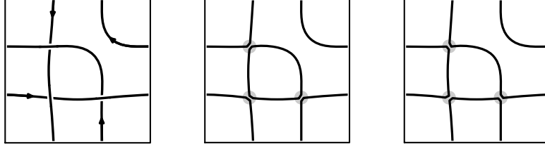
FIGURE 14. A minimal genus diagram of the virtual Borromean rings in the torus, and the states S_A and S_B .
