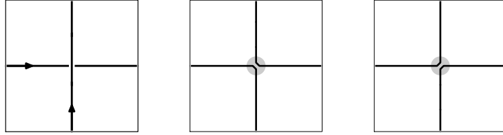
FIGURE 13. A minimal genus diagram of the virtual Hopf link in the torus, and the states S_A and S_B .
