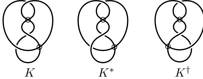
FIGURE 18. The virtual knot K = 3.1 and its mirror images.
