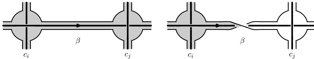
FIGURE 10. The band \beta connecting the disk at c_i to the disk at c_j . Since the crossings are opposite (over/under), the band will be untwisted if the smoothings are the same ( AA or BB ) and twisted if the smoothings are opposite ( AB or BA ).
