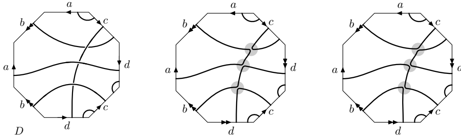
FIGURE 19. A minimal genus diagram of 3.1 and the states S_A and S_B .
