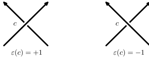
FIGURE 3. A positive and a negative crossing.
