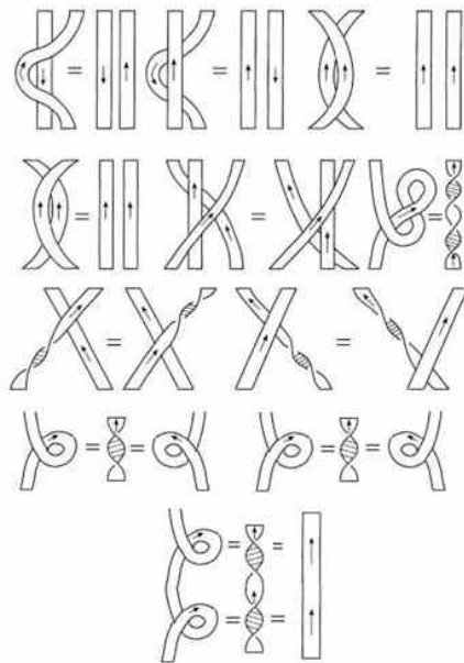
Figure 3: Relations between tangle generators
