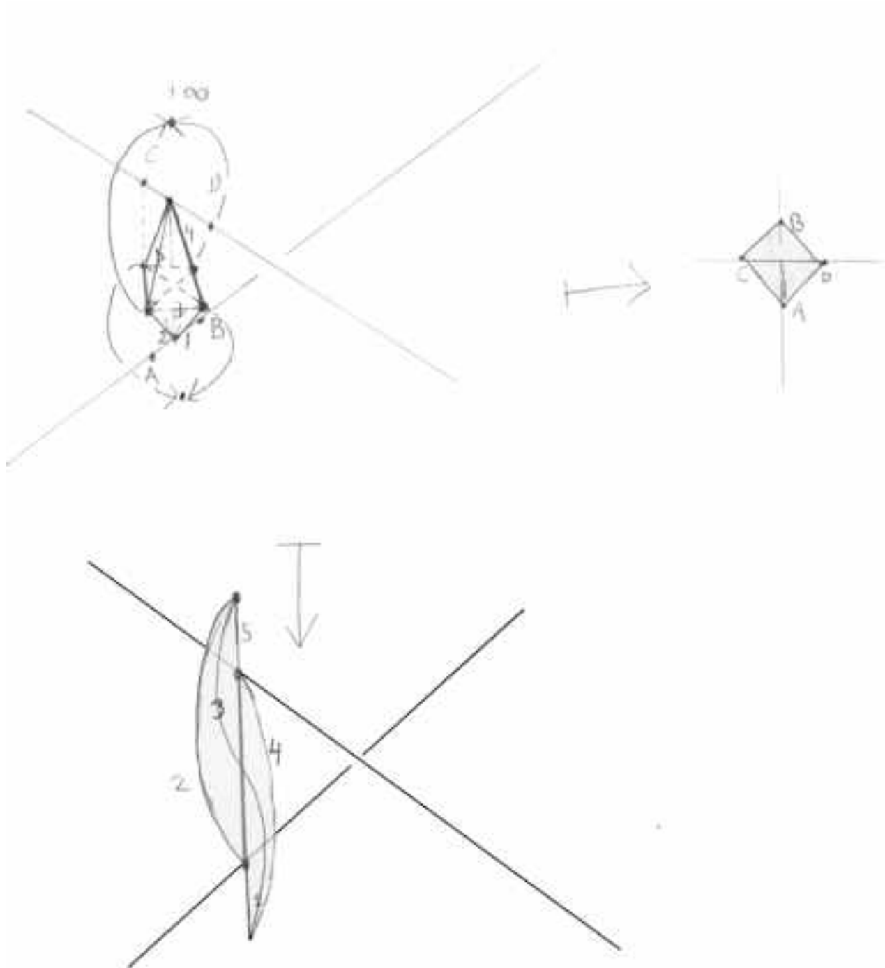
Figure 14: At top left, one of the octahedra O_\nu . At top right, the projection of O_\nu onto D before we've dragged the vertices. At bottom, one of the tetrahedra obtained from O_\nu , after having its vertices pulled to \pm\infty .
