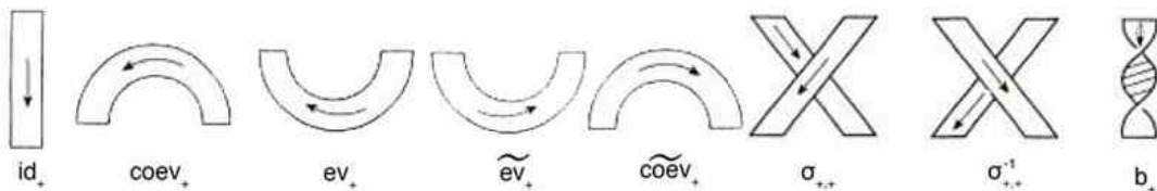
Figure 2: Structure morphisms for +
