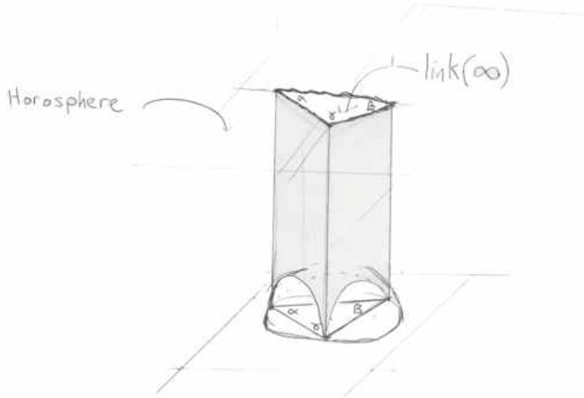
Figure 9: An ideal tetrahedron in U^3 , intersecting a horosphere about \infty (i.e, a Euclidean plane), to form its link L(\infty) , with dihedral angles \alpha, \beta, \gamma
