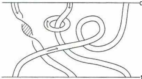
Figure 1: Diagram of a (3,3) oriented ribbon tangle, or “ribbon”
