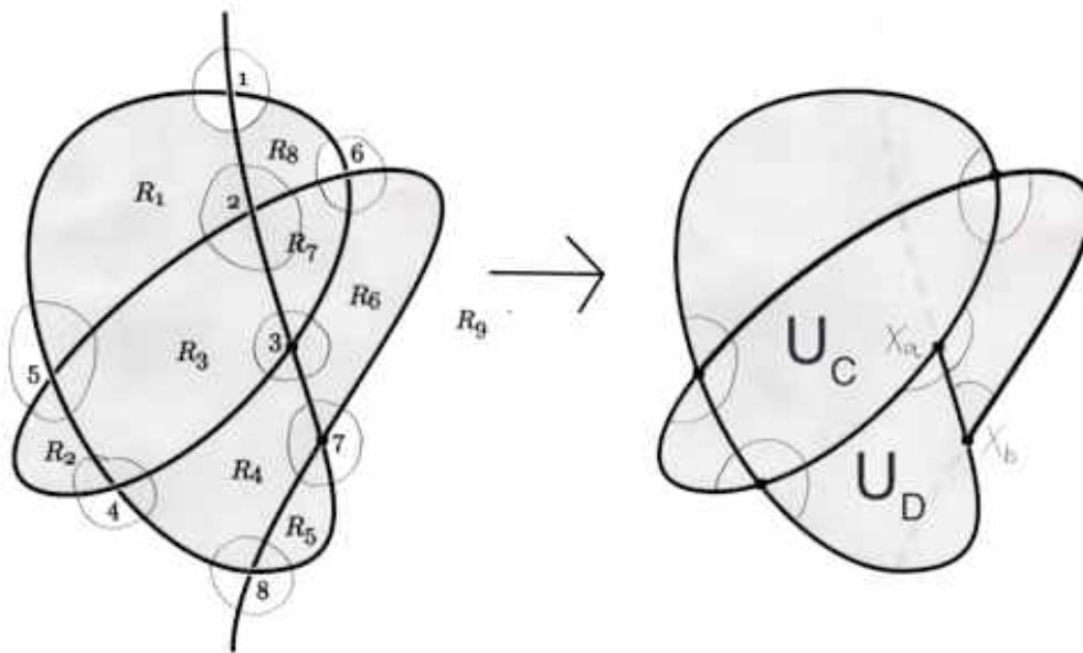
Figure 19: The angles indicated at the right correspond to the tetrahedra which have survived the degeneration. U_c and U_d are the faces which contain the two missing arcs, and abut the trivalent vertices.
