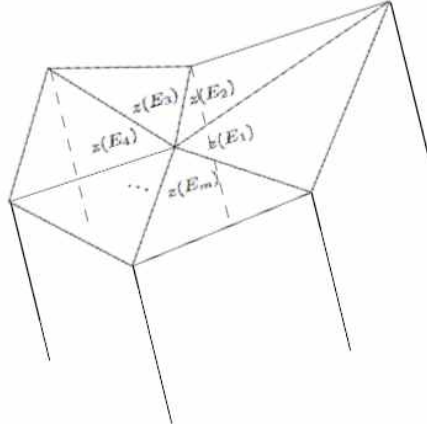
Figure 12: Links of tetrahedra fitting around an edge
