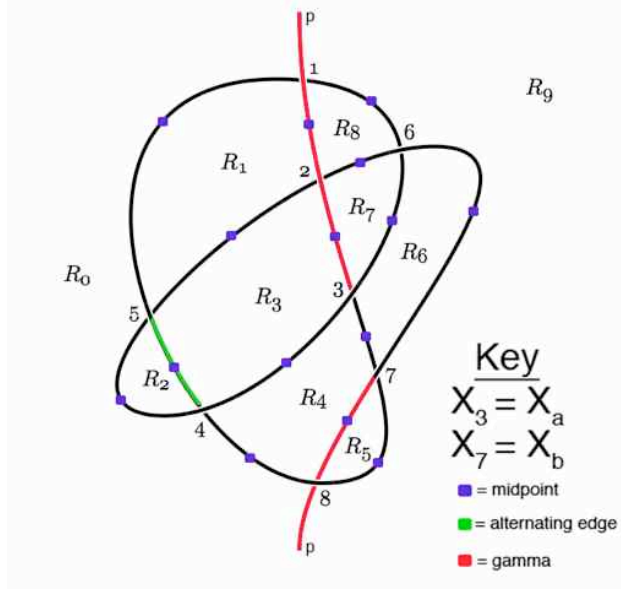
Figure 13: The knot 8_{21} , which we will use as our example. We've labeled an example of an alternating edge, as well as the midpoints, and the arc \gamma .
