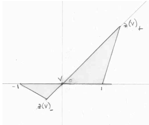
Figure 10: z_+(v) is for the positively oriented case, z_-(v) the negatively oriented case.
