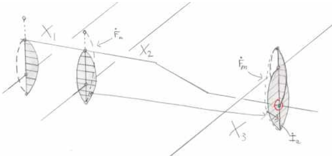
Figure 22: \dot{F}_m , in U_c , collapsing to I_\alpha .
