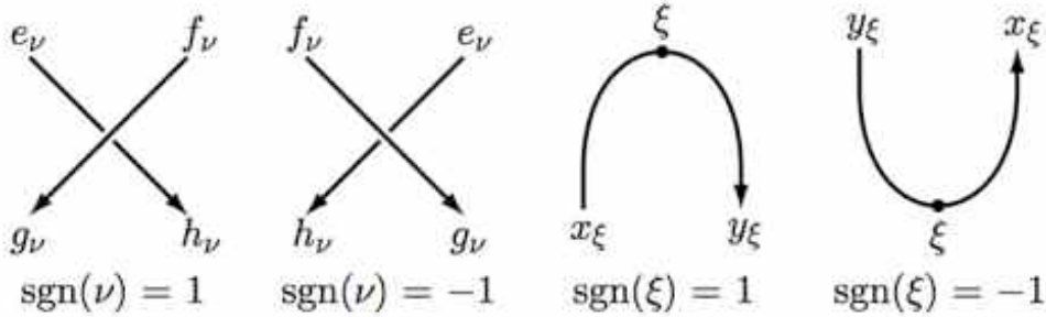
Figure 31: Signs for vertices
