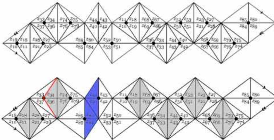
Figure 26: Triangulation of the knot L by \hat{S}
