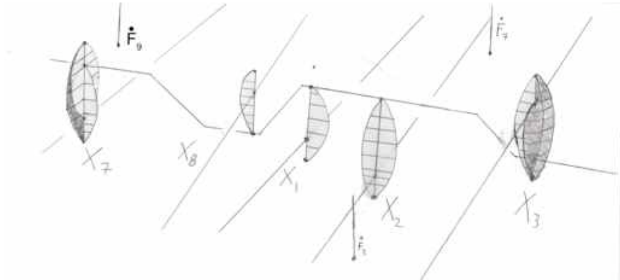
Figure 18: Crossings labeled as in Figure. 13. Remark that there are only 3 non-degenerate tetrahedra in the picture; two from X_3 = X_a , but only one from X_7 = X_b , because it is adjacent to \dot{F}_9 = \dot{F}_{n+1} , as we have drawn.
