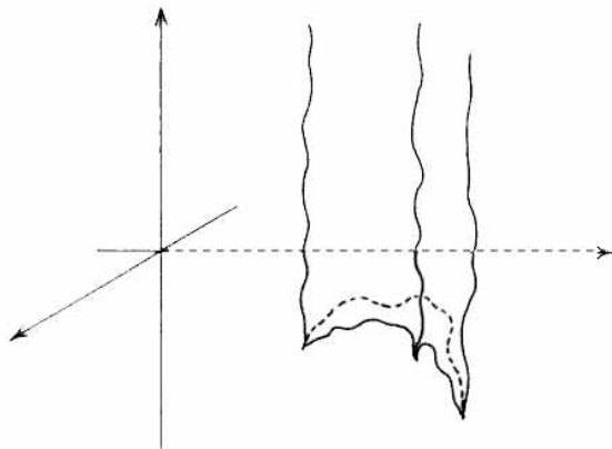
Figure 11: A positively oriented topological tetrahedron (pictured in U^3 ) whose straightening will be negatively oriented
