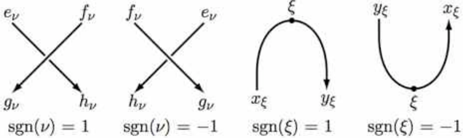
Figure 7: Signs for vertices
